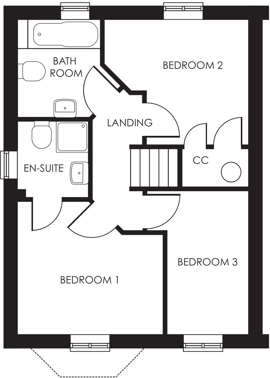
FIRST FLOOR
