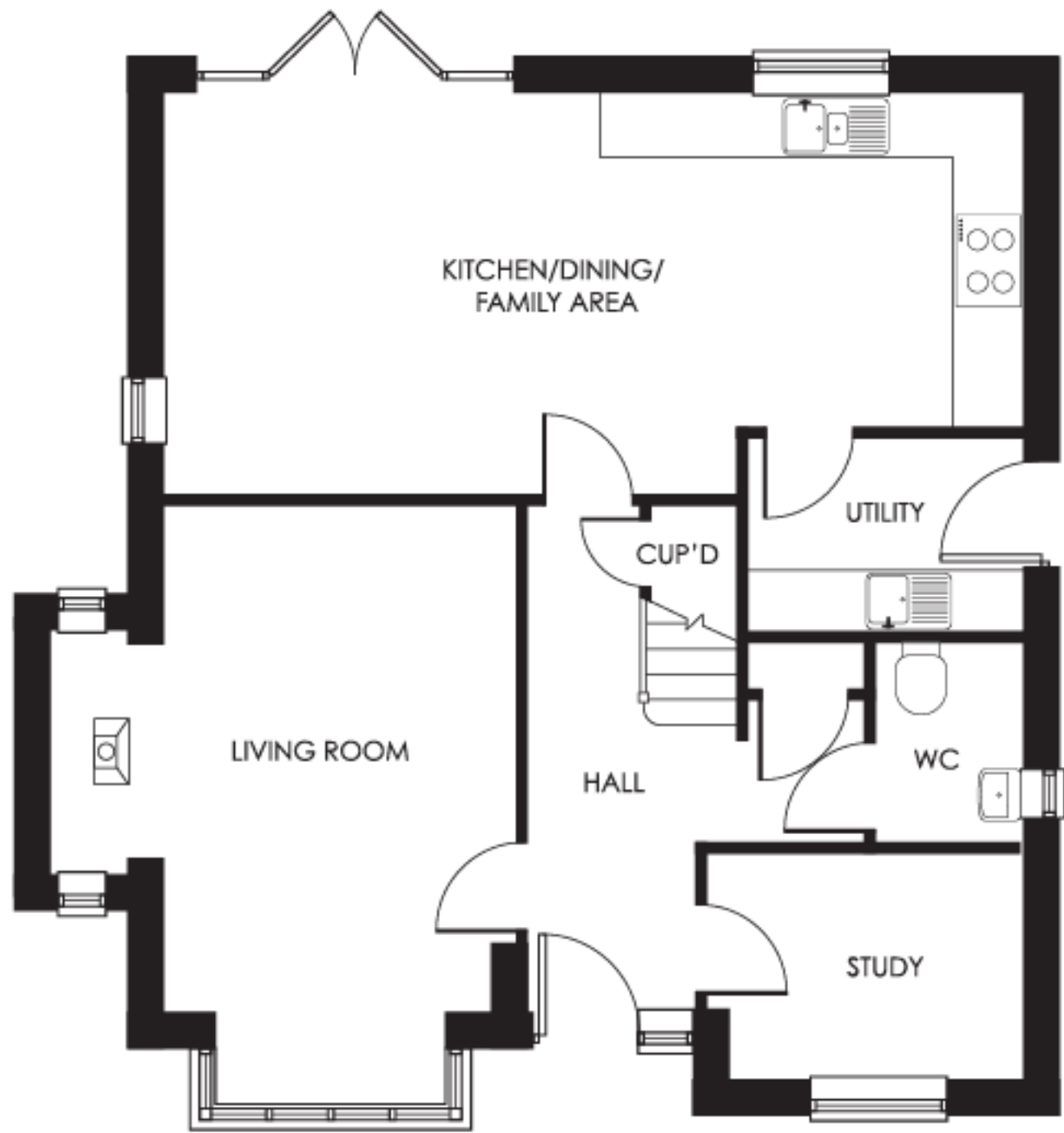
GROUND FLOOR
