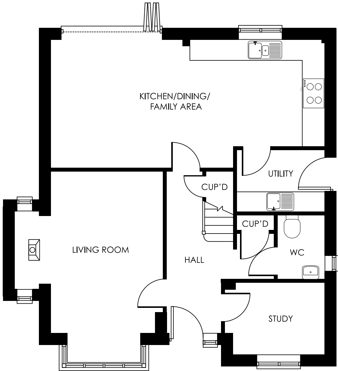
GROUND FLOOR
