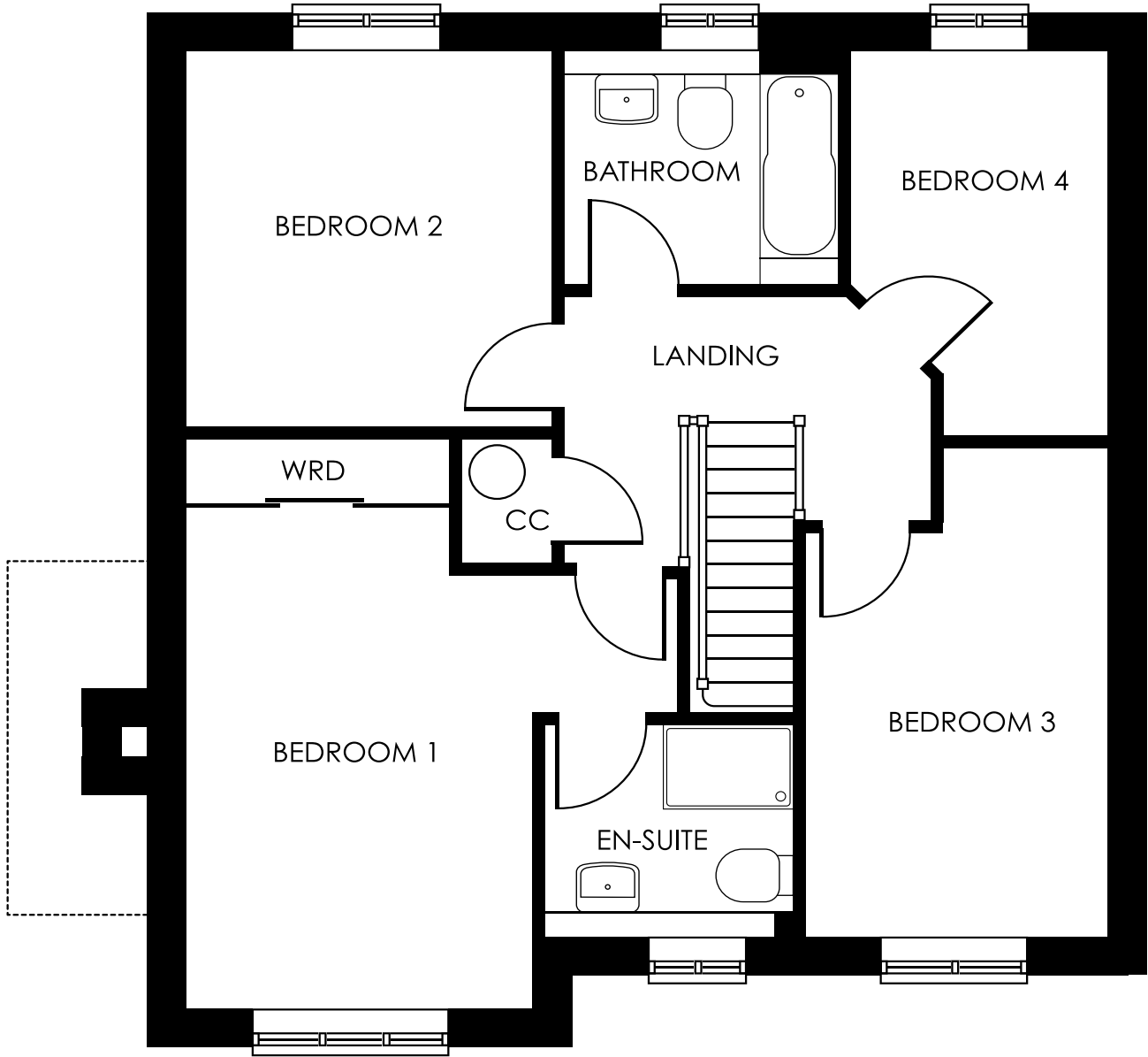
FIRST FLOOR
