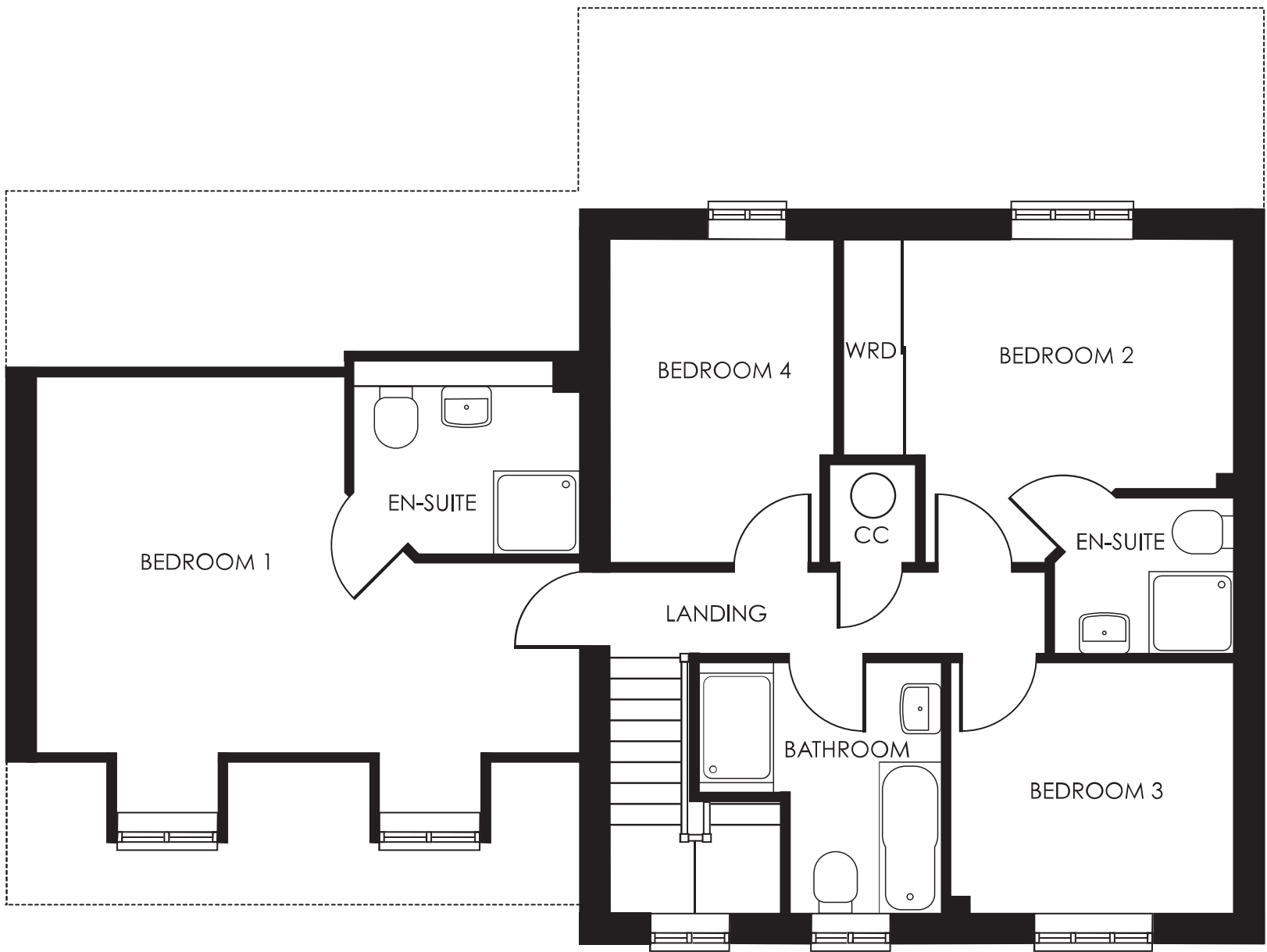
FIRST FLOOR
