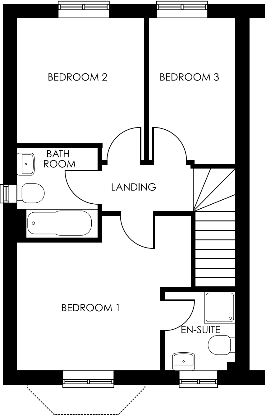
FIRST FLOOR
