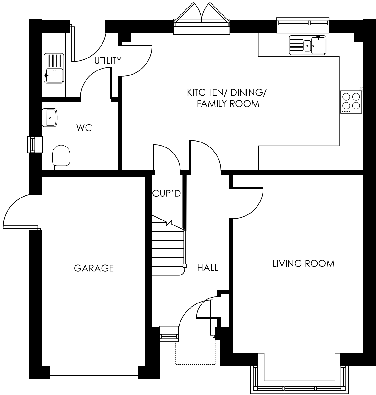
GROUND FLOOR
