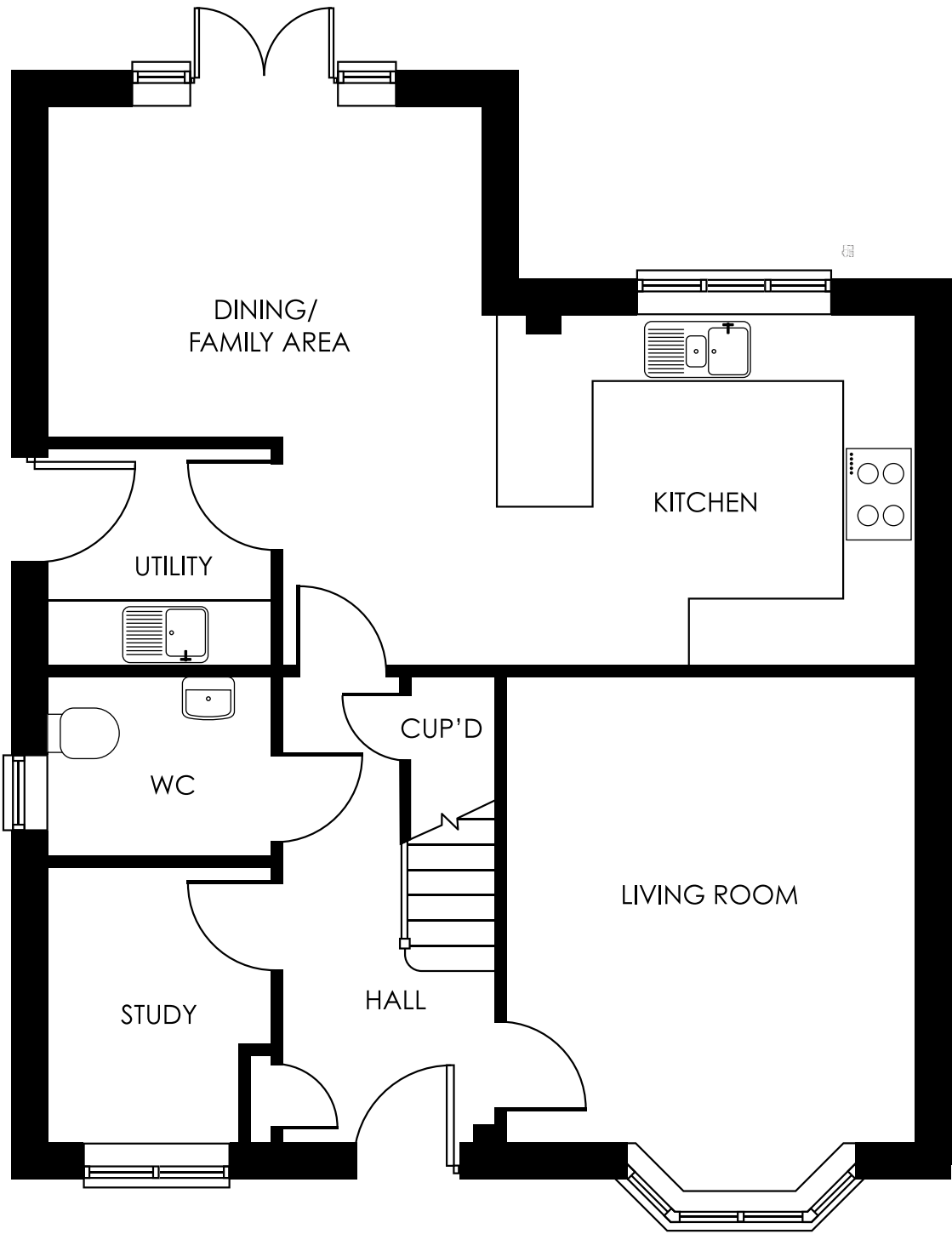
GROUND FLOOR
